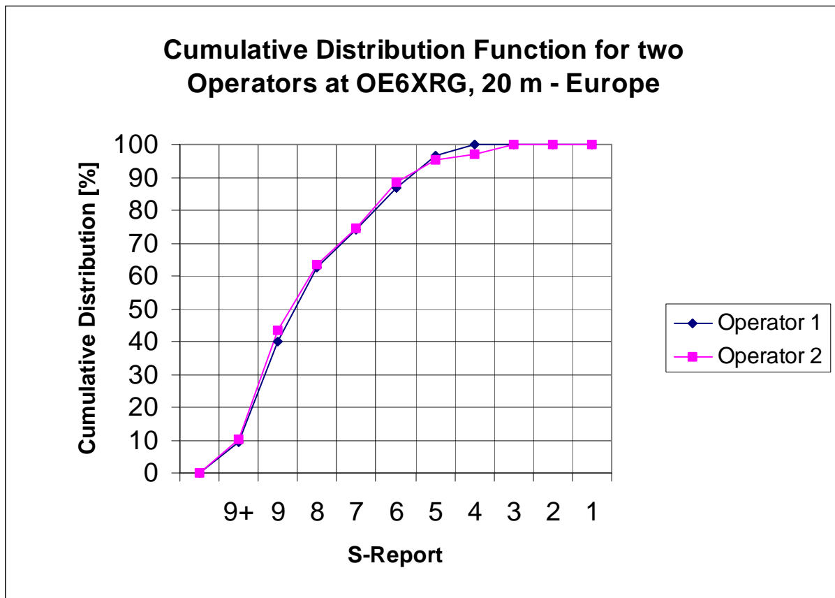
Fig. 2: Cumulative distribution function for club station OE6XRG, 20 m Europe
