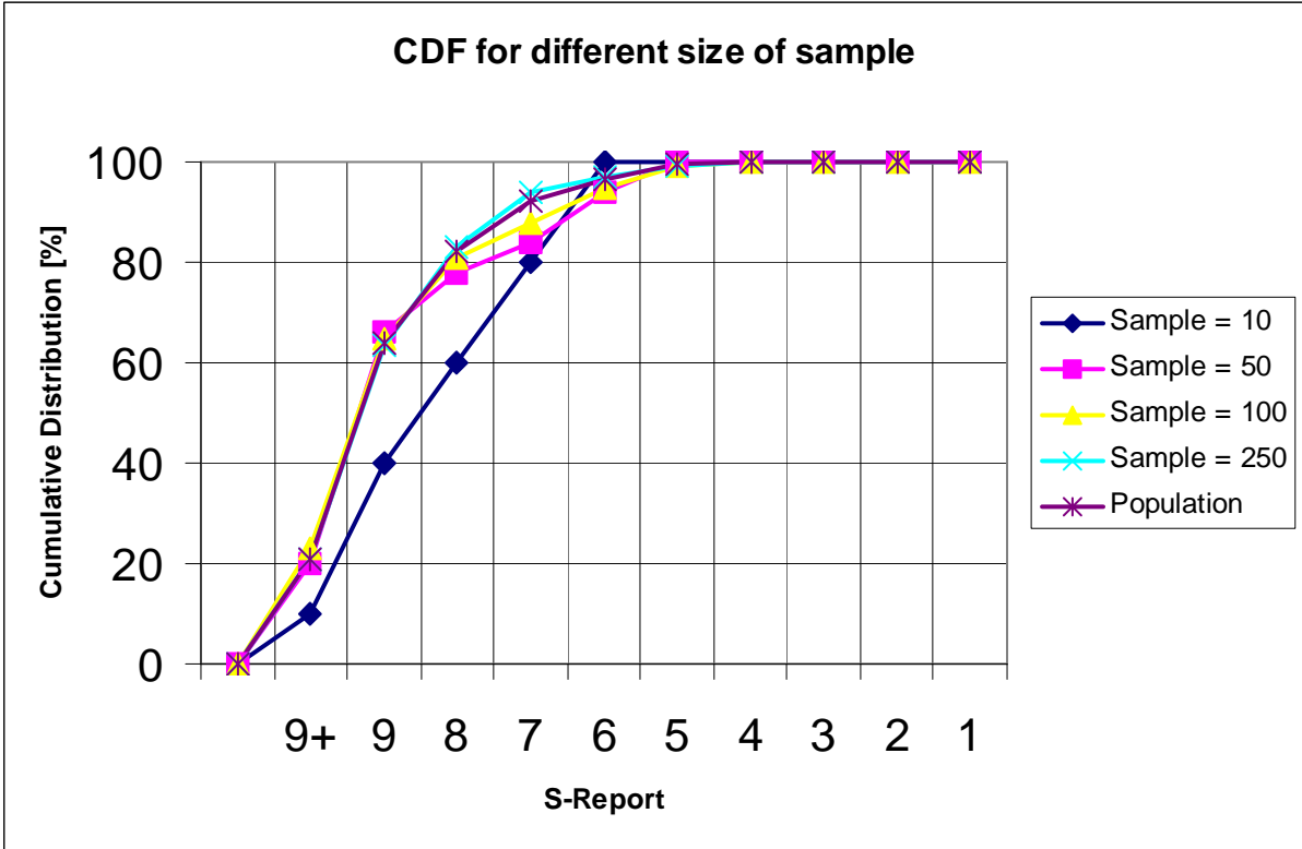
Fig. 3: Cumulative distribution function for different sample size
